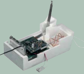
The radiosonde electronics for measuring temperature, moisture content and air pressure are protected in a polystyrene housing.
