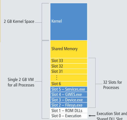
Comparison of the address space under Windows CE 5.0 and 6.0
