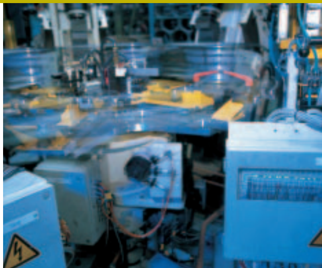
The automation components are connected with each other via a Lightbus system.
